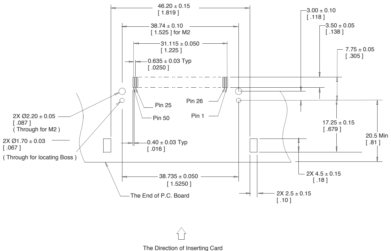
Recommended PCB Solder Pad Pattern
